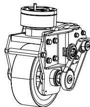
12. Drive Motor
