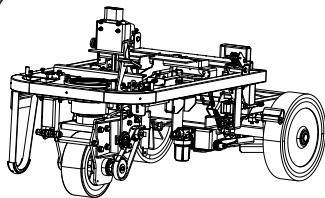
11. Chassis
