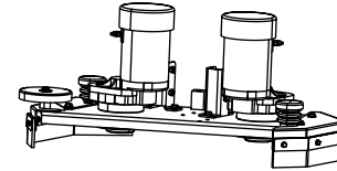
4. Brush Head - 750
